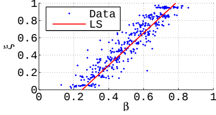
Figure 2. Values of the spatial interpolator \xi as a function of the relative similarity \beta , given by (6), for many training query images sampled along lines connecting image map images. Notice the affine dependence of \xi on \beta .
